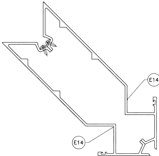
MULLION 'MC'
