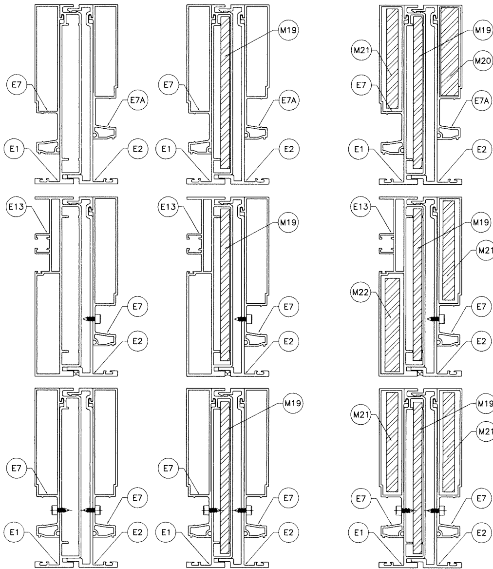
MULLION 'M1'
