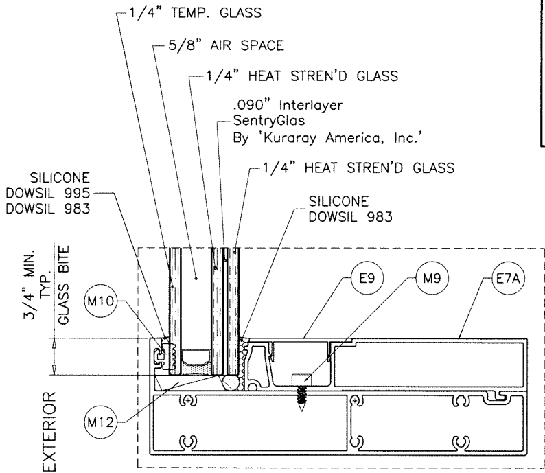
GLASS TYPE 'C' 1-7/16" OVERALL INSUL. LAM. GLASS
