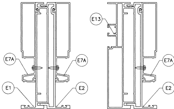
MULLION 'M1C'
